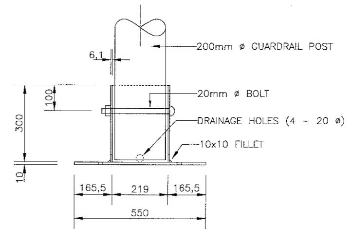
SECTION X-X
