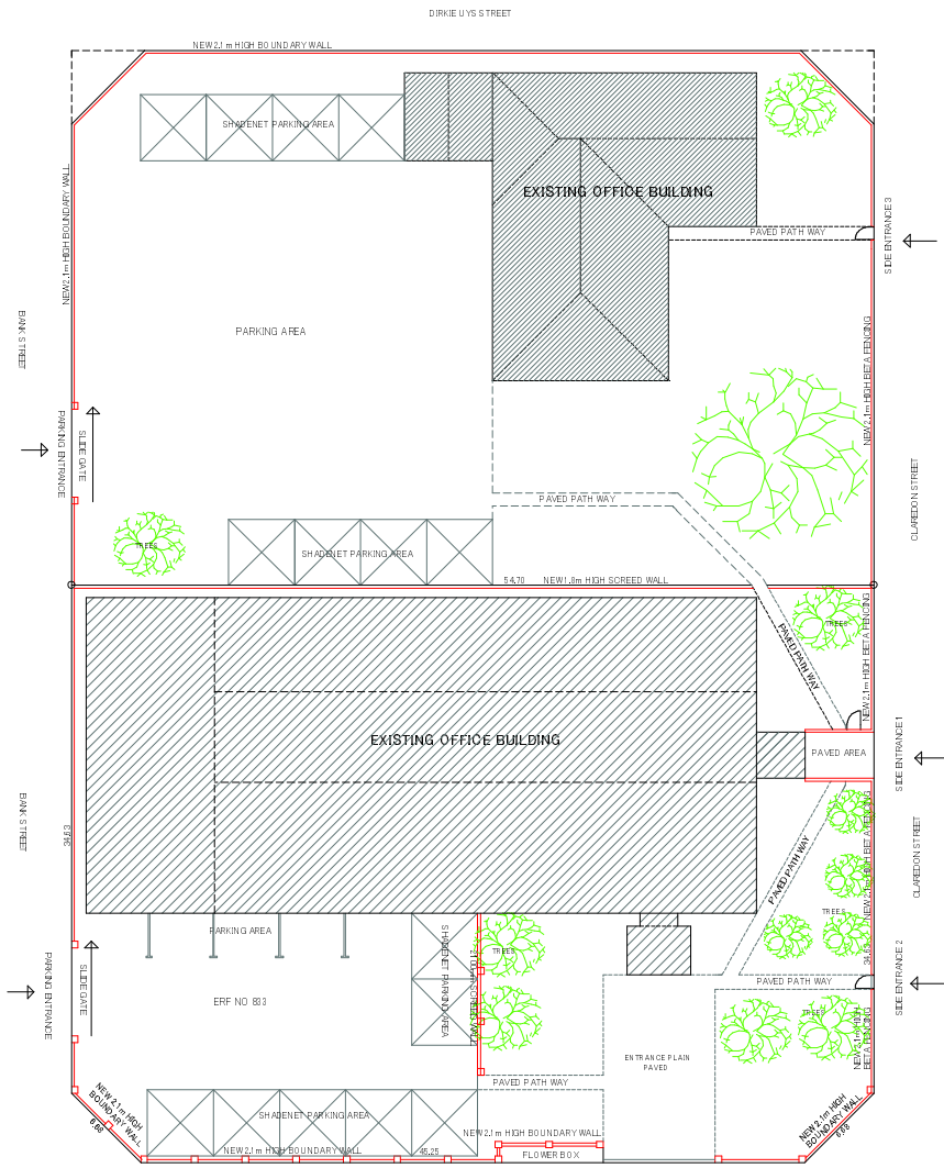
:SITE LAYOUT :SCALE 1:200
