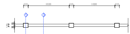
:PLAN VIEW :SCALE 1:50
