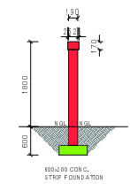
:SCREED WALL DETAIL :SCALE 1:50
